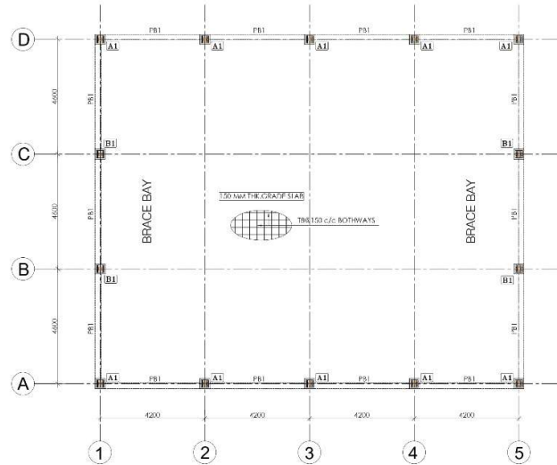
PLINTH BEAM LAYOUT PLAN
