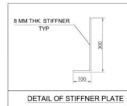
DETAIL OF STIFFENER PLATE
