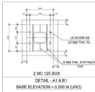
ANCHOR BOLT LAYOUT PLAN
