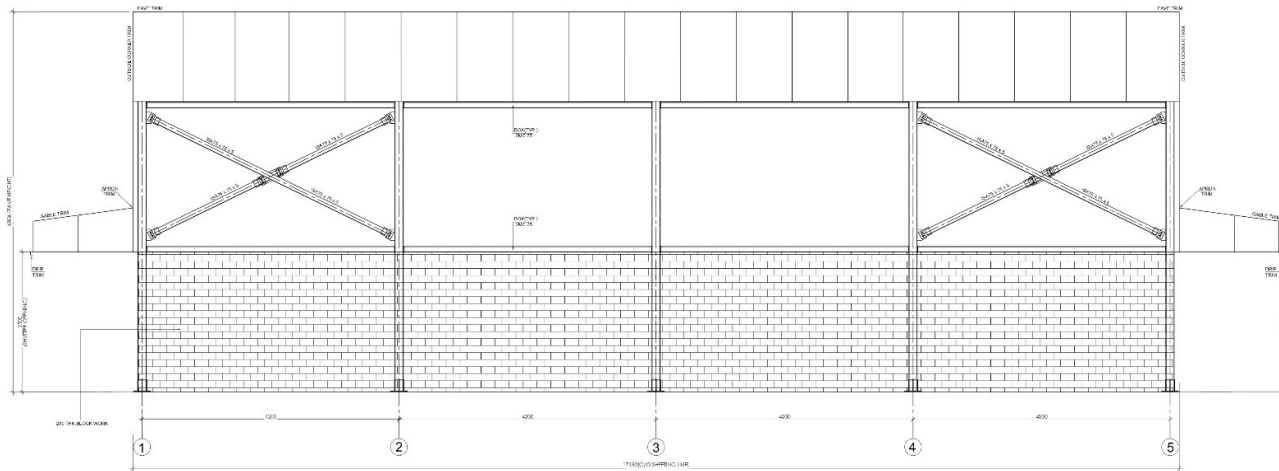
SIDE WALL SHEETING ELEVATION @ GRID LINE A & D
