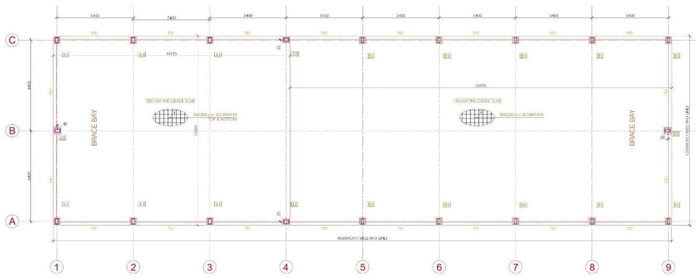
PLINTH BEAM LAYOUT PLAN (Concrete Pads are as per preferred locations & as per our design)
